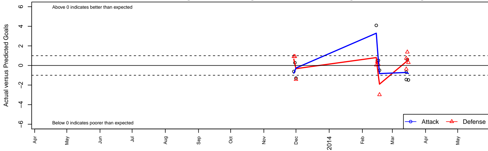
SC del Sol 96 B95 Dots are actual minus expected GF (blue circles) and GA (red triangles). Blue line is smoothed change in attack strength. Red is smoothed change in defense strength.
